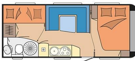
Hobby De Luxe 545 KMF Model 2015
